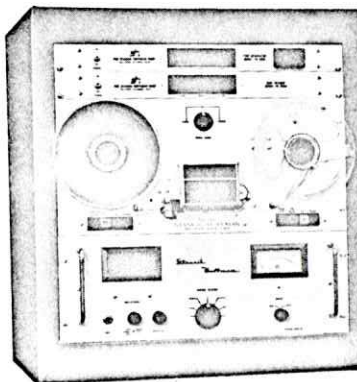
CRM-7 Recorder/Reproducer with Digital time and high speed automatic search. (Size 19" x 19")
